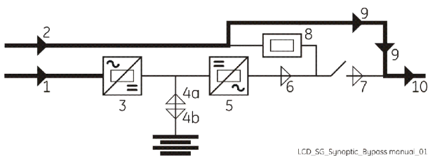
LCD_SG_Synoptic_Bypass manual_01
