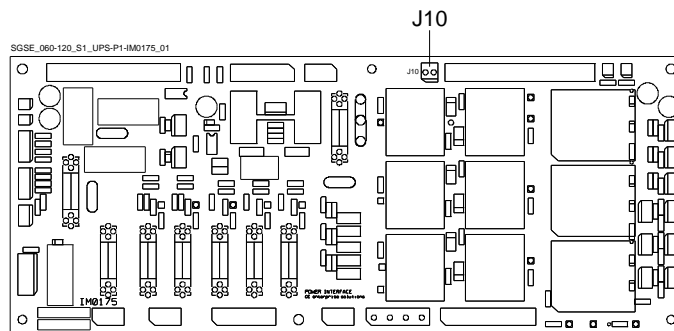
P1 - Power Interface
