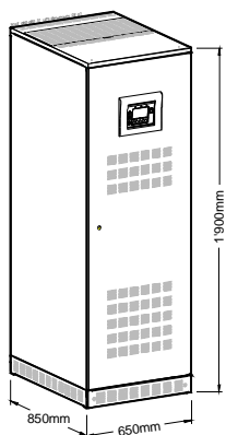
SG-CE Series 100 – 120кВА PurePulse®
