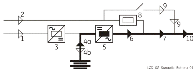
LCD_SG_Synoptic_Battery_01
