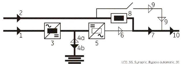
LCD_SG_Synoptic_Bypass automatic_01
