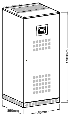
SG-CE Series 100 – 120кВА PurePulse®
